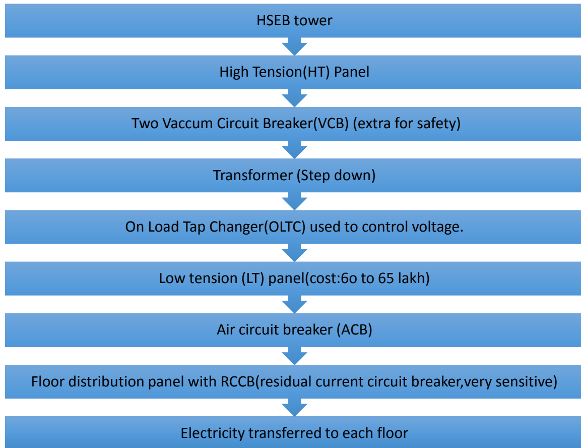
Figure 2.1.2: Electricity transfer flowchart
